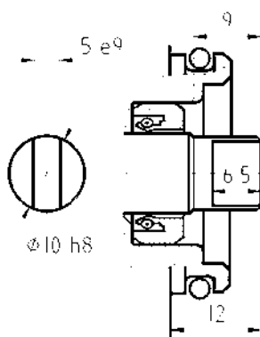
Coppia max 18 Nm Max torque 18 Nm
