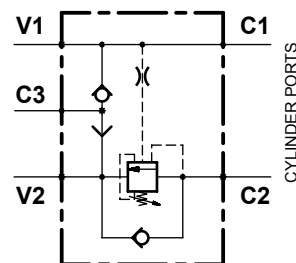
Schema Idraulico / Hydraulic Scheme :
