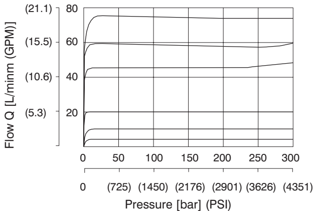
TV2-102/MC Meter-in compensator
